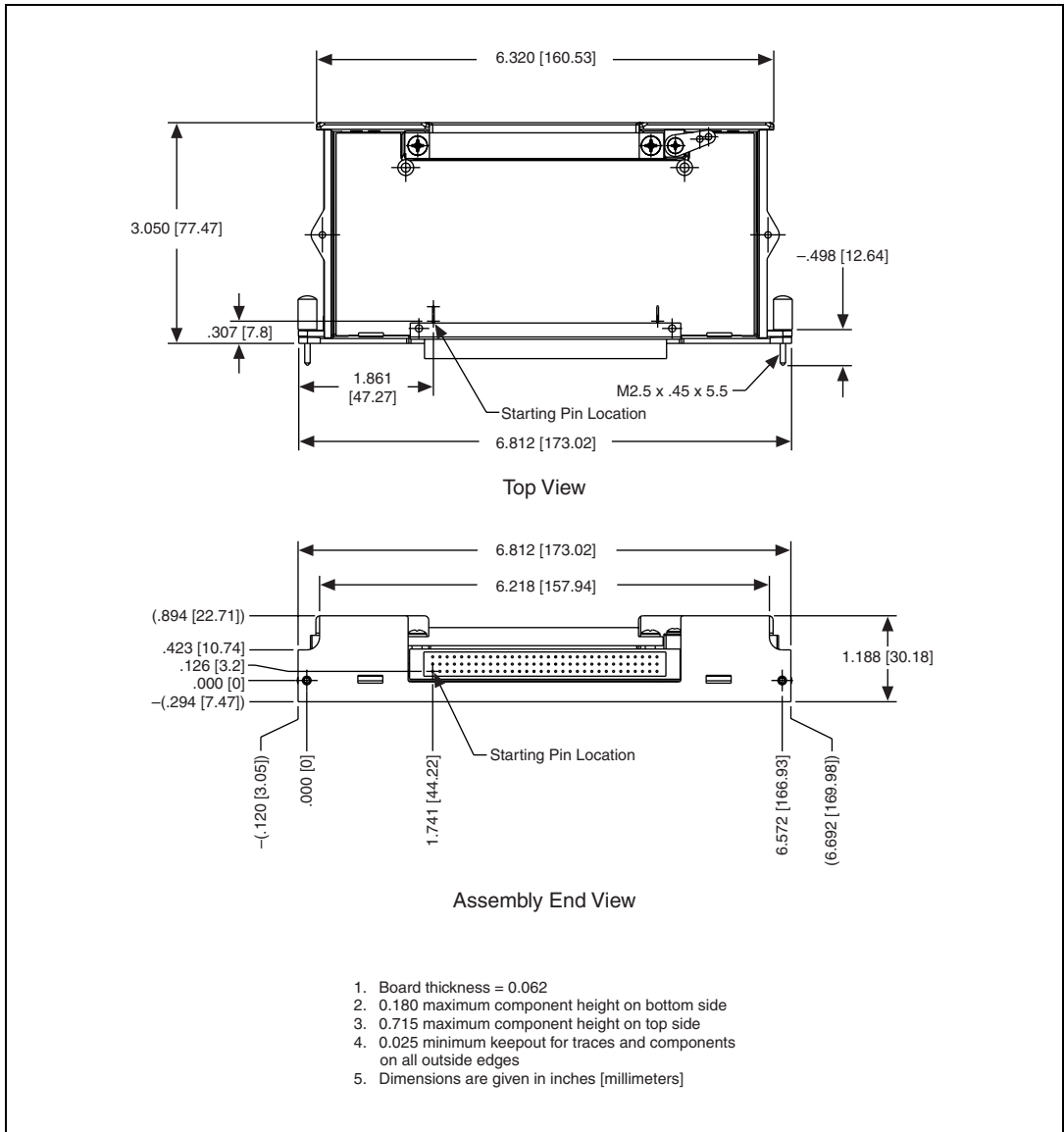
Figure 1. SCXI-1381K Dimensions
